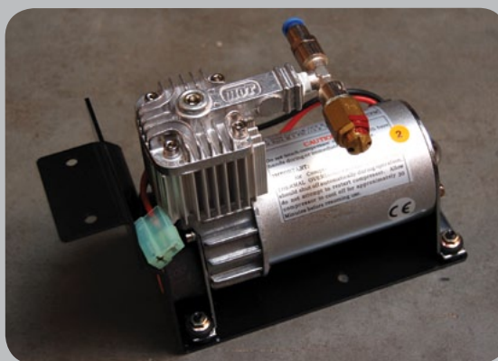
Compressor
